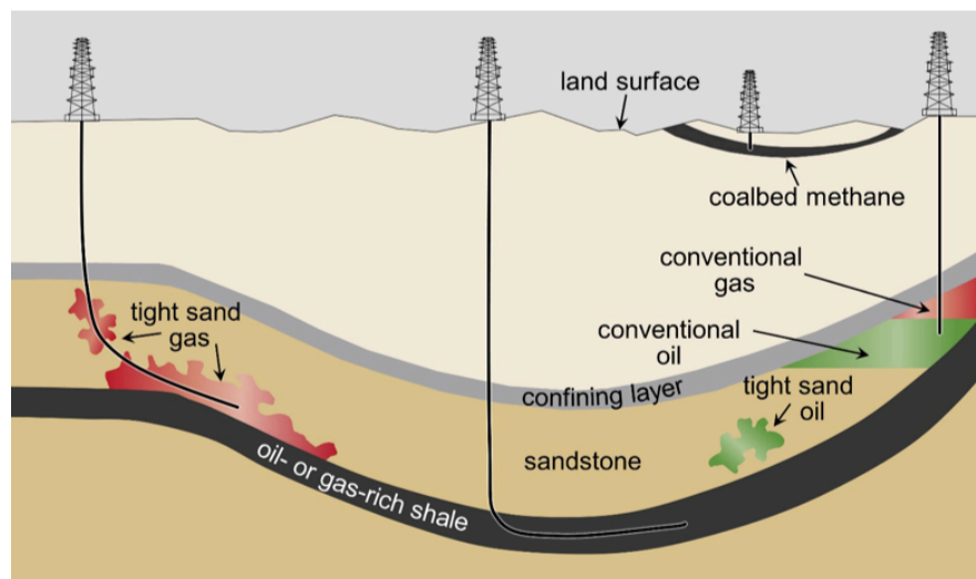
Figure 2. Shown are conceptual illustrations of types of oil and gas wells. A vertical well is producing from a conventional oil and gas deposit (right). In this case, a gray confining layer serves to "trap" oil (green) or gas (red). Also shown are wells producing from unconventional formations: a vertical coalbed methane well (second from right); a horizontal well producing from a shale formation (center); and a well producing from a tight sand formation (left). Note: Figure not to scale. 2
