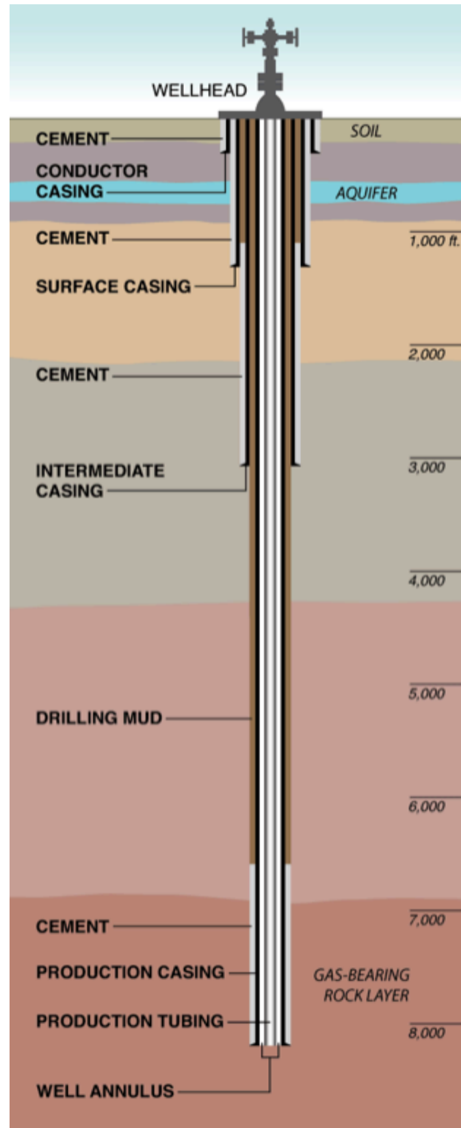
Figure 4. Several layers of steel casing typically enclose a well bore through ground water aquifers. The empty spaces between can be sealed with cement. Note: Figure not to scale. Graphic by Al Granberg, ProPublica.
